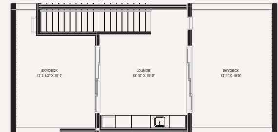
LEVEL FOUR AND ROOFTOP SKYDECK
