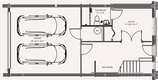
LEVEL ONE
