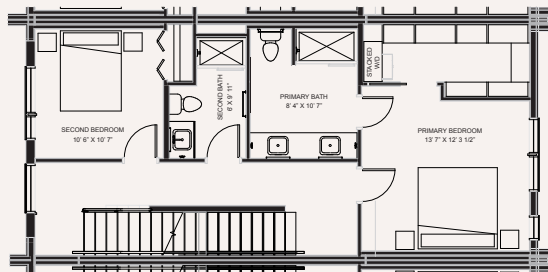
LEVEL THREE
